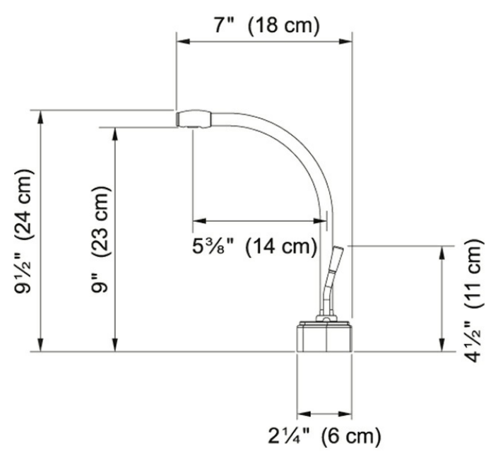
Technical Drawing
