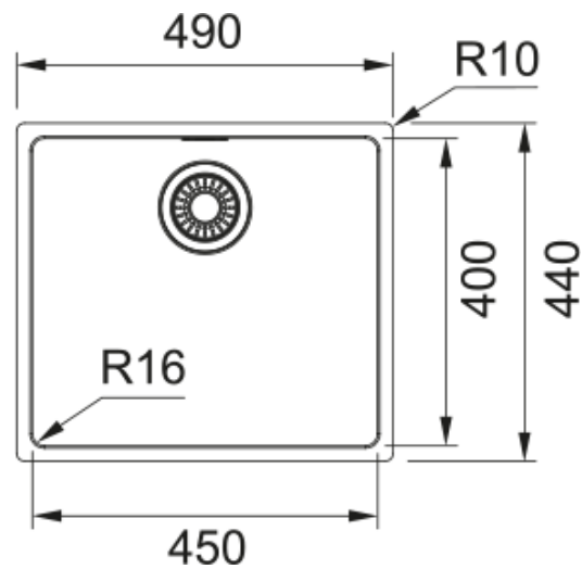
Maris MRX110-45 Single Bowl Sink 490x440mm Undermount, Stainless Steel Satin Finish. 90mm Waste. 25 Year Warranty.
