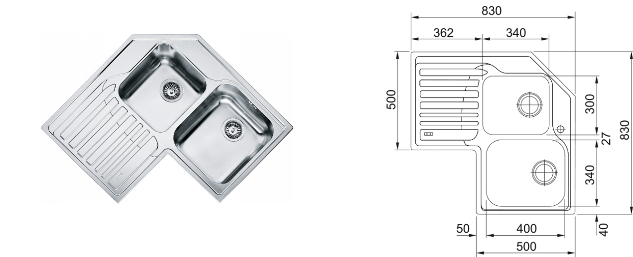
Studio STX621 830x830mm, Left Hand Drainer, Inset, Stainless Steel. 90mm Waste. 25 Year Warranty.
