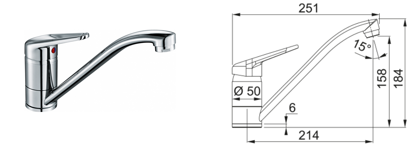
Tap Novara Plus, spout, top lever, high pressure, chrome, G 3/8" 450mm hose
