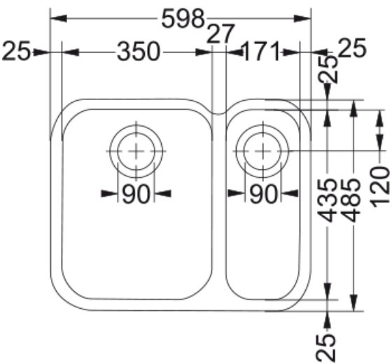
ARIANE ARX 160-D 598x485mm, Undermount, Right Hand Small Bowl, Silk Stainless Steel, 3½" Semi-Integrated Wastes with Hygienic Overflow. 50 Year Guarantee on all Franke sinks.
