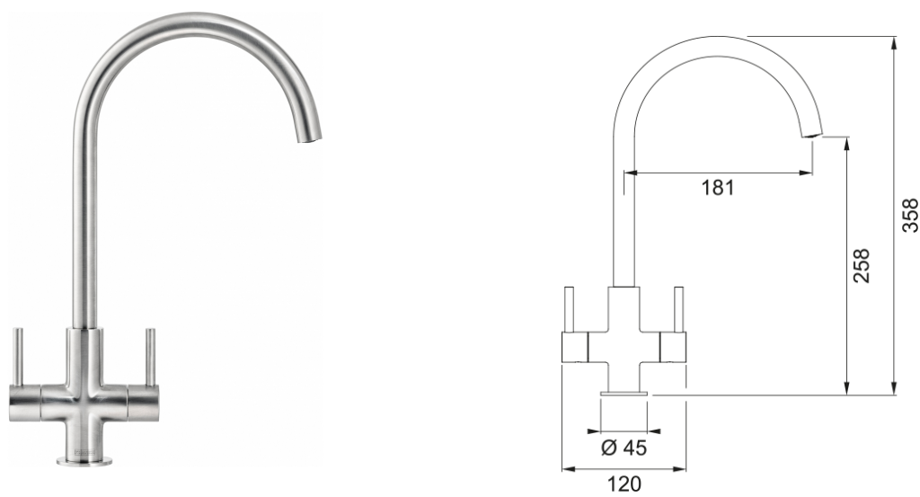
Hestia J-Spout SilkSteel tap, Overall height 358mm, twin lever, Ceramic valves.
