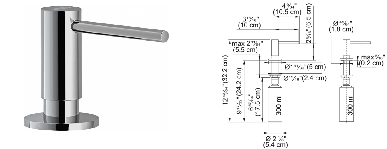
SD902 Soap Dispenser Active Chrome 300ml.
