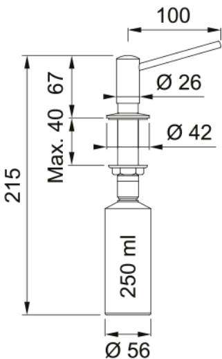
Soap dispenser Novita stainless steel for bore from 18mm up to 35mm with bottle 250ml
