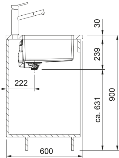
Maris Single Bowl Stainless Steel Satin Finish Sink MRX110-55. 90mm Waste. 25 Year Warranty.
