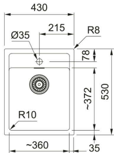
SID 610-40 430 x 530mm 3 1/2" with basket strainer waste kit with round overflow tap hole carbon
