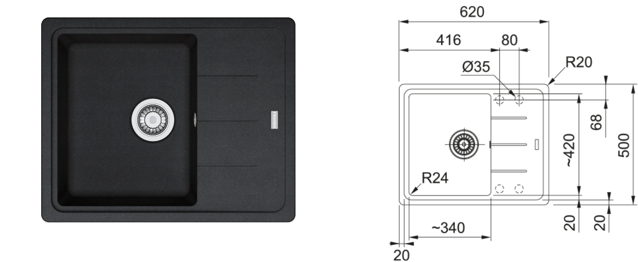
BFG 611-62 620x500mm, reversible, onyx, with basket strainer waste twist control 3 1/2" and overflow
