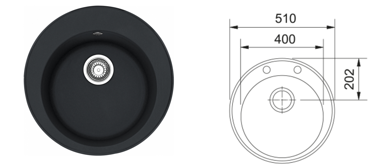
ROG 610-40 diameter 510mm, , 3 1/2", with waste kit, with siphon, without drainer, ONYX
