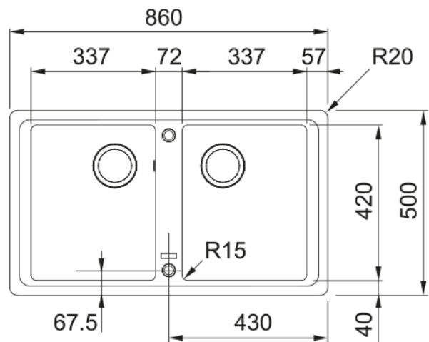
BFG 620 860x500mm, onyx, 3 1/2", with overflow, with waste kit, with siphone, Franke Brand
