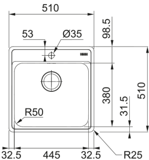
BCX 610-51 510x510mm, stainless steel brushed, 3 1/2" waste hole, with waste kit, with overflow hole and with tap hole, Chinese label
