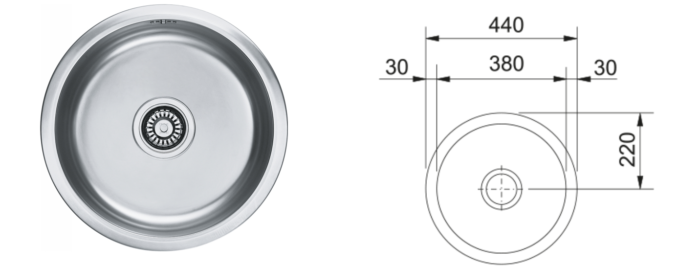
LUT 610, 440x440mm, no drainer, stainless steel microtexture with basket strainer waste twist control 3 1/2" and cut out template and carton and plastic colander and clips
