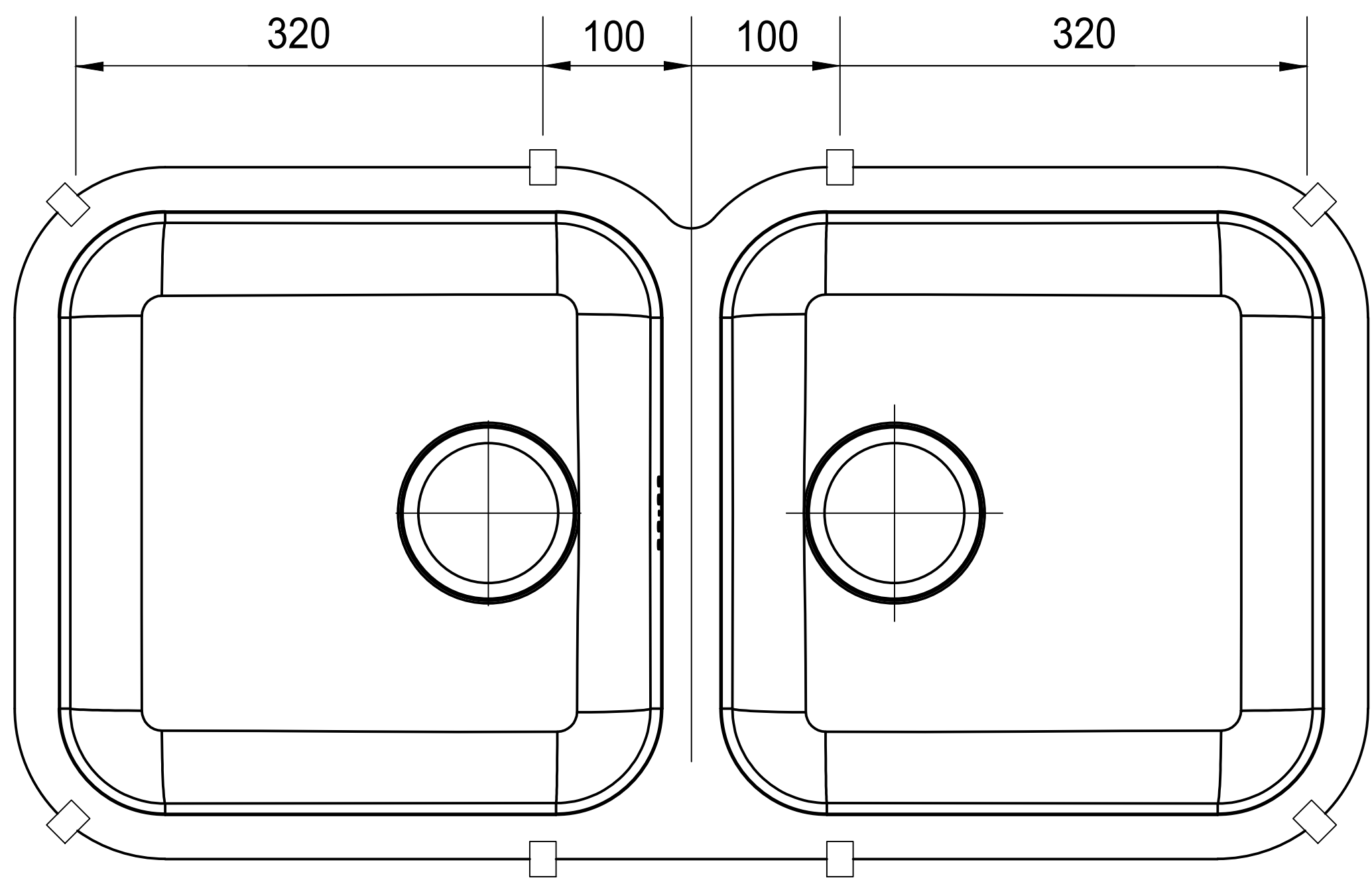
Recommended fixing clamps position
