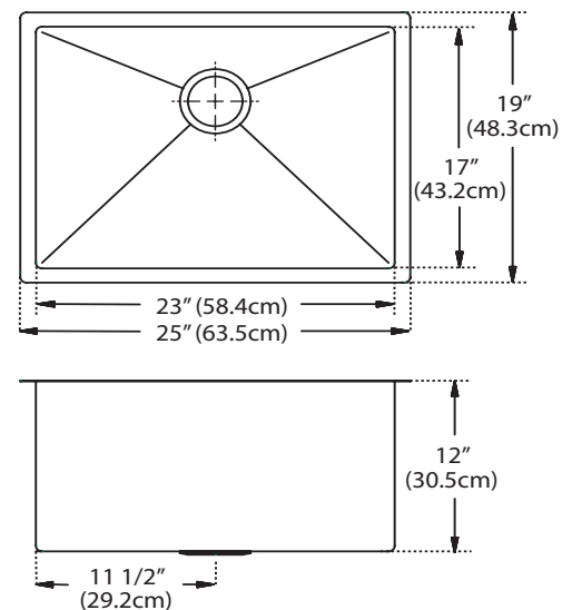
Dimensional Drawing
