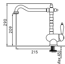
Modell Eos Neo utdragbar pip m dusch, rostfri
