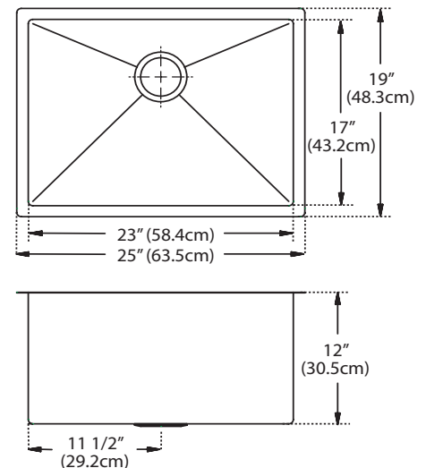
Dimensional Drawing
