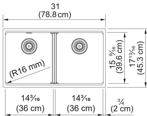
Dimensional Drawing
