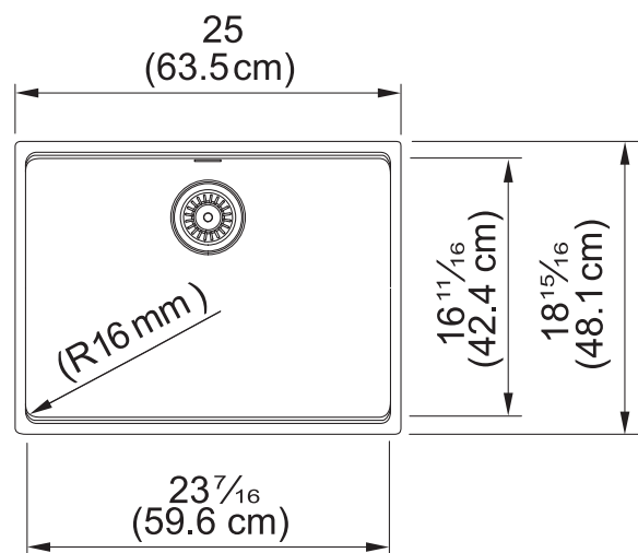
Dimensional Drawing
