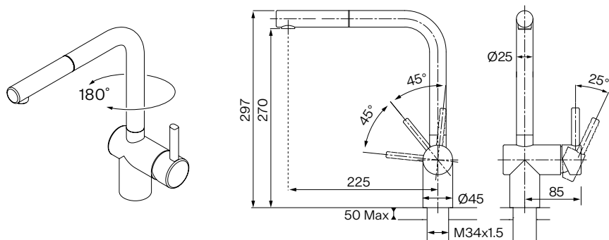
Tap Atlas Neo Nozzle side HP SS Version
