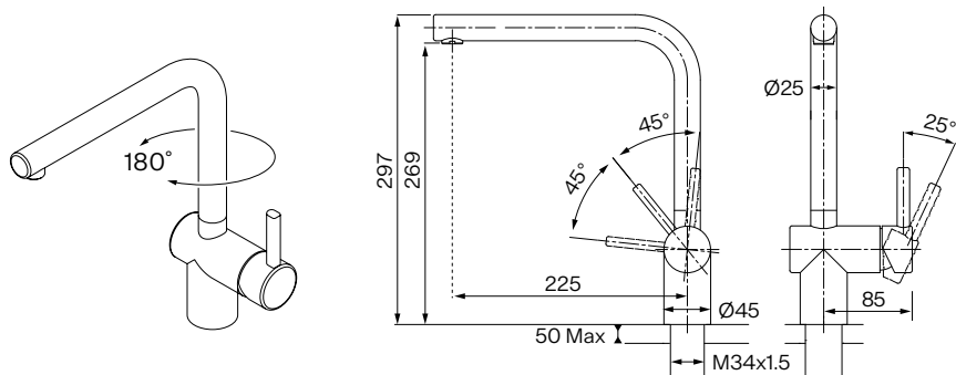
Tap Atlas Neo Swivel Side HP SS Version
