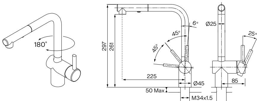
Tap Atlas Neo Pull Out Spray HP SS
