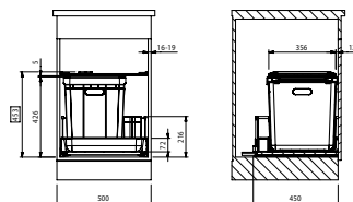
Model Sorter 350-50
