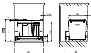
Model Sorter 350-60
