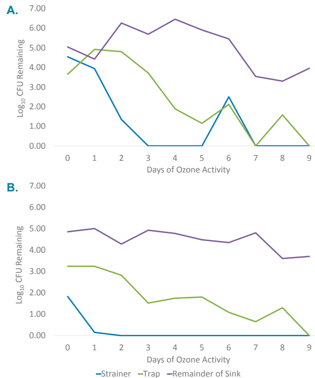
Figure 1. A) Elimination of Pseudomonas sp. from the ozone sink B) Elimination of C. auris
