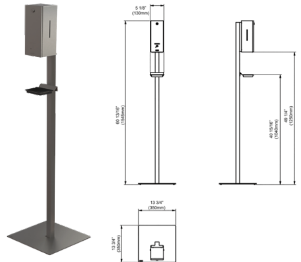
STD37 Slim stand shown with RODX627H dispenser
