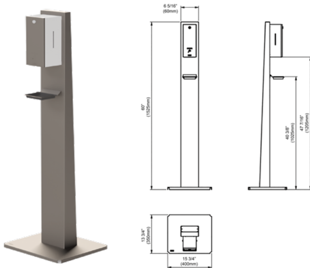
STD36 Stand shown with RODX627H dispenser
