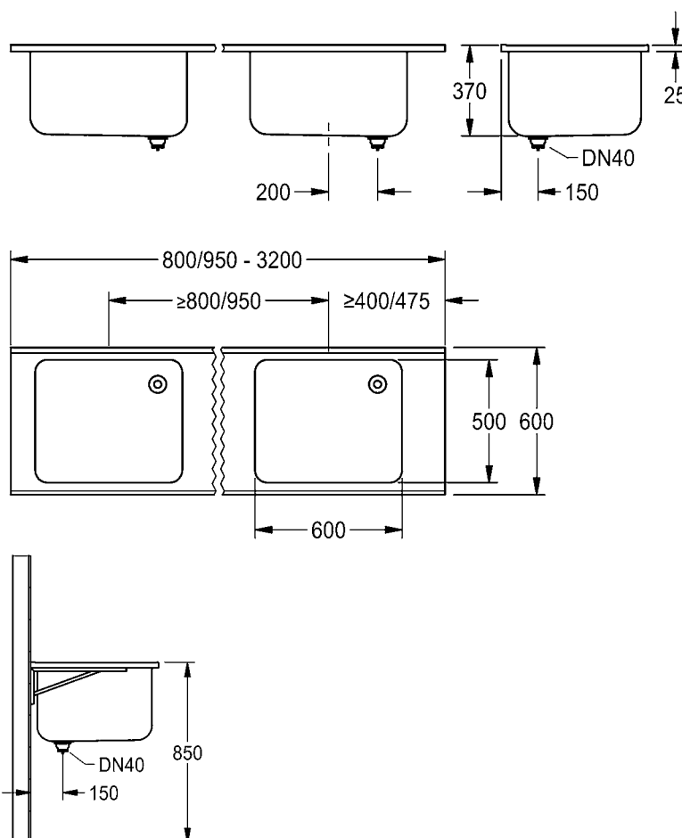
Example of VARIUSmed multi-purpose washbasin with laterally positioned bowl
