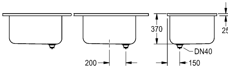
Example of VARIUSmed multi-purpose washbasin with laterally positioned bowl
