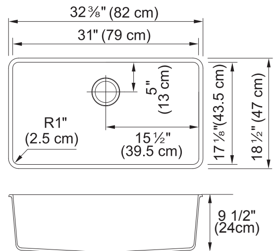
Dimensional Drawing
