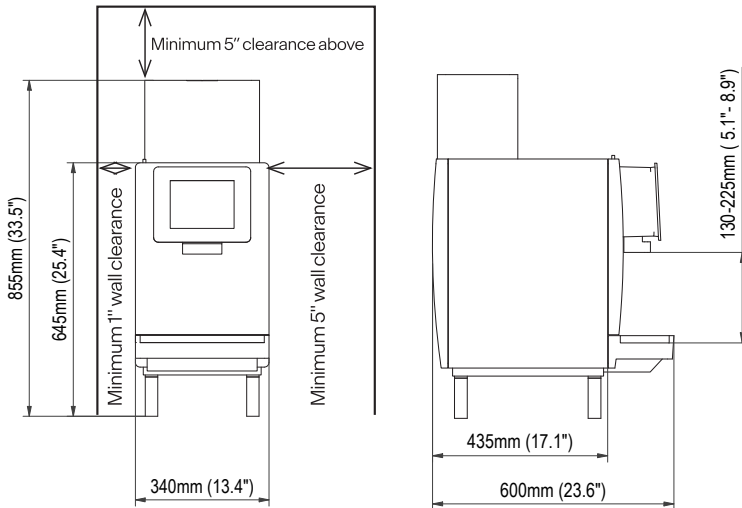
Standard Configuration - Front Profile
