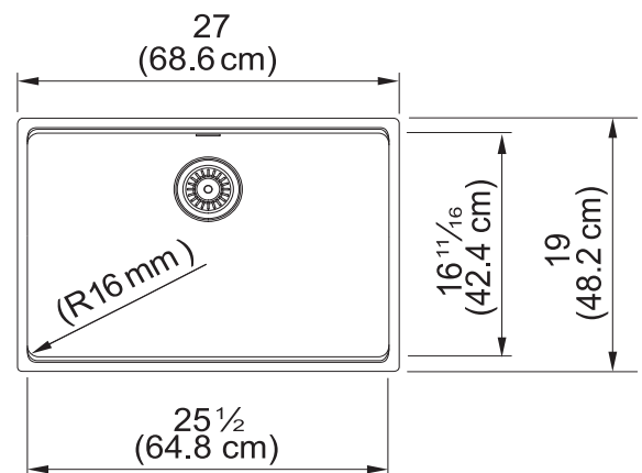
Dimensional Drawing
